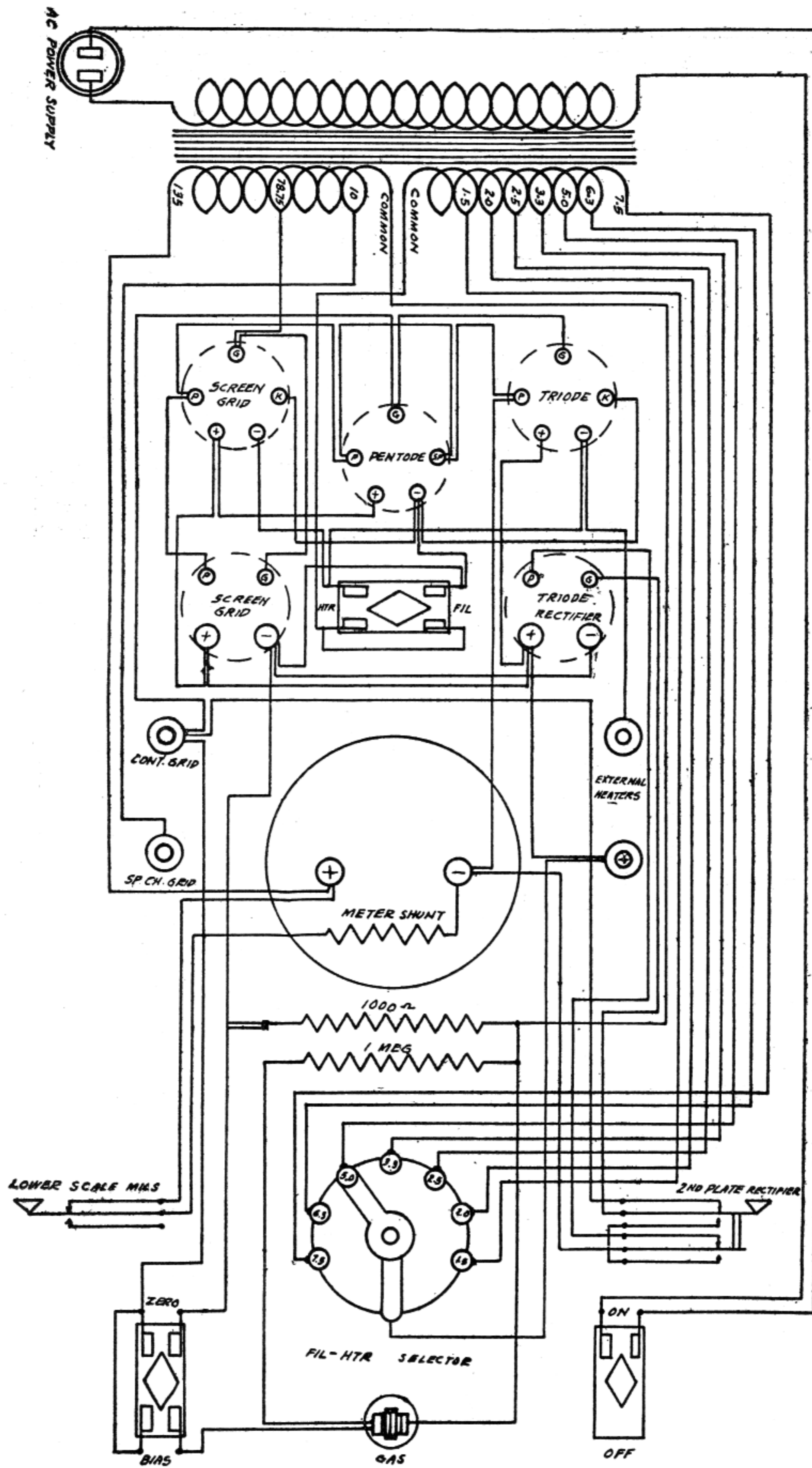
SUPREME INSTRUMENTS CORP. MODEL 40 Tube Checker
