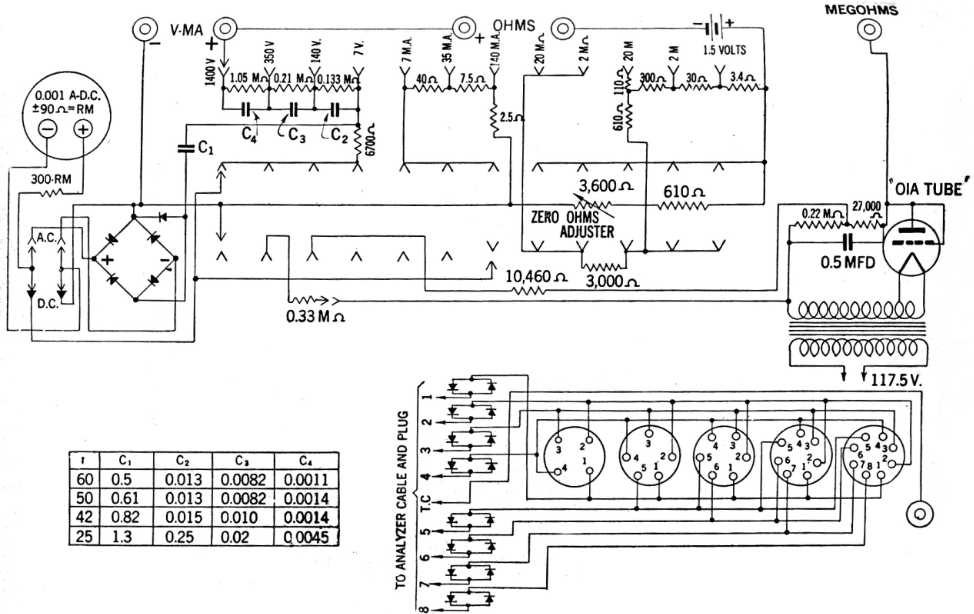
FIG. 27—Wiring diagram of Supreme Model 551 analyzer.
